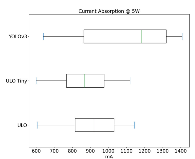
Fig. 6. The current absorption distribution of three models when running in the 5 W power profile.
